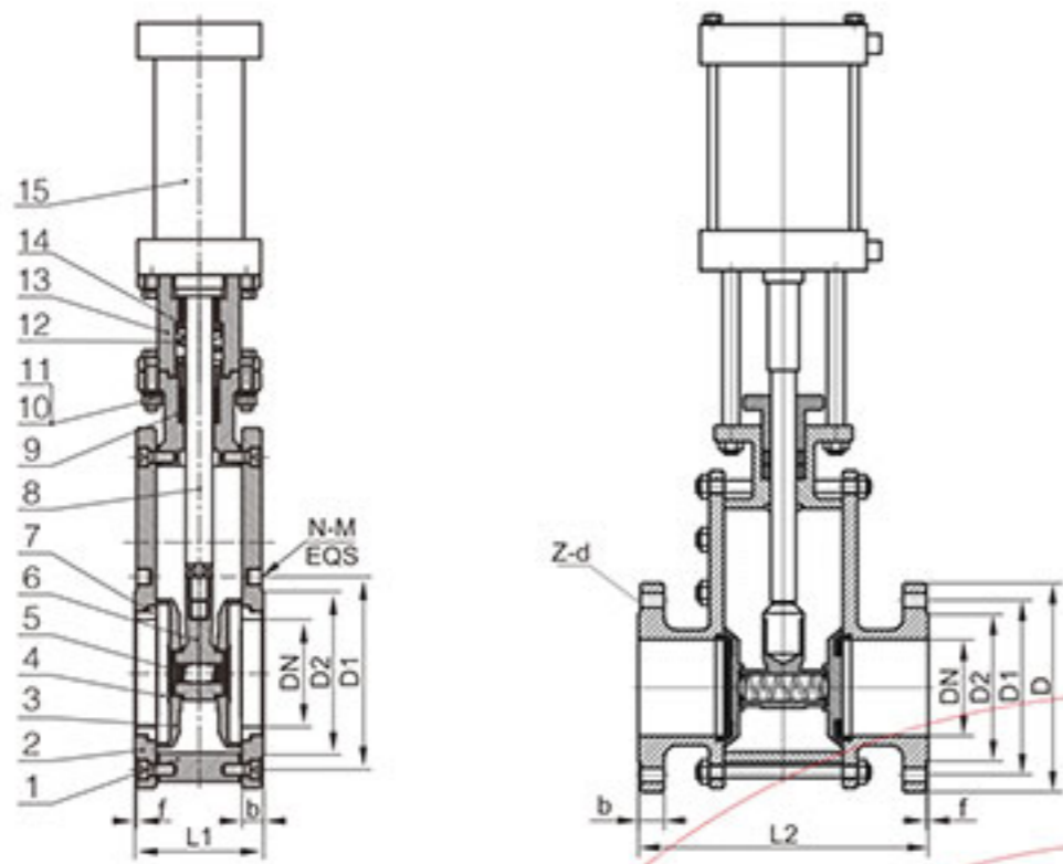
气动陶瓷双闸板阀 Pneumatic Ceramic Dual-plate Ceramic Valve
